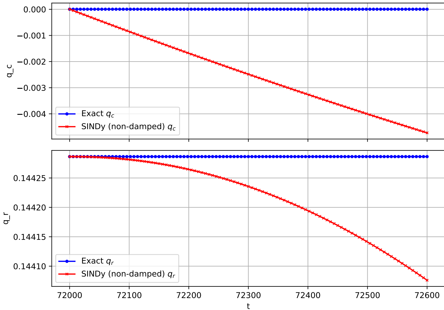
Trajectory 908 (non-damped)
