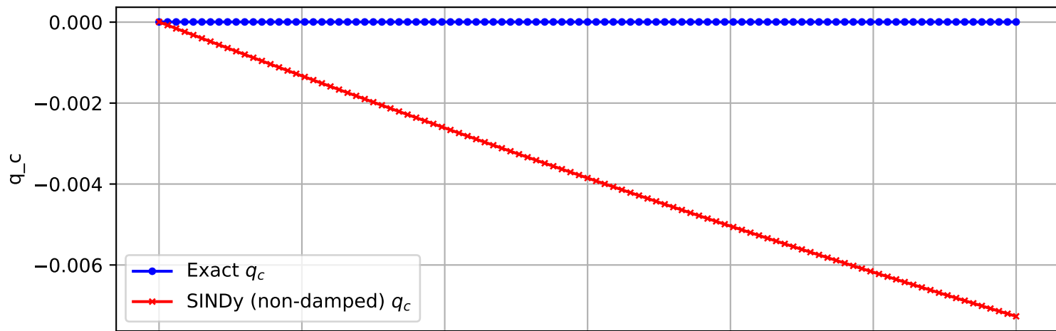
Trajectory 918 (non-damped)
