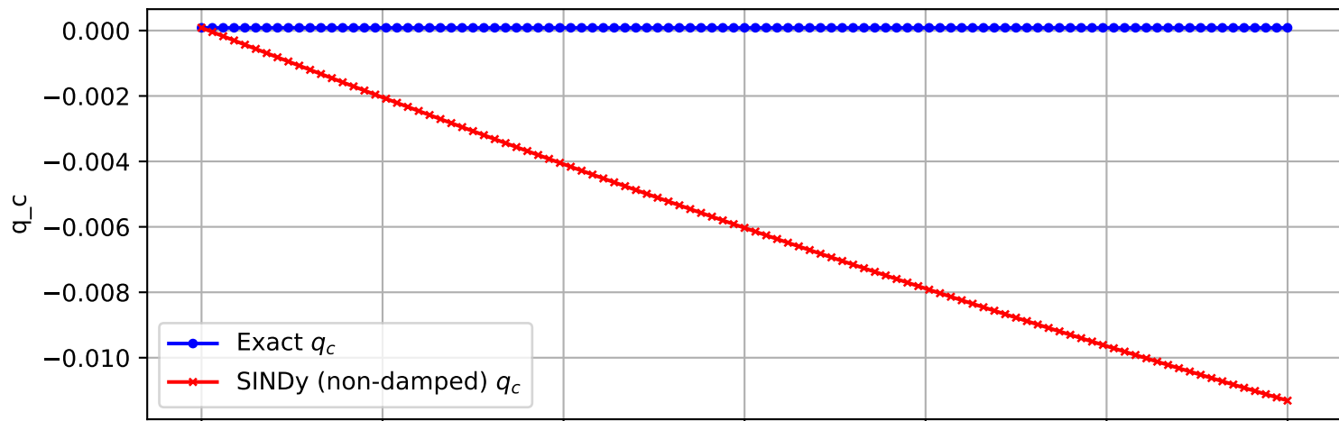
Trajectory 933 (non-damped)
