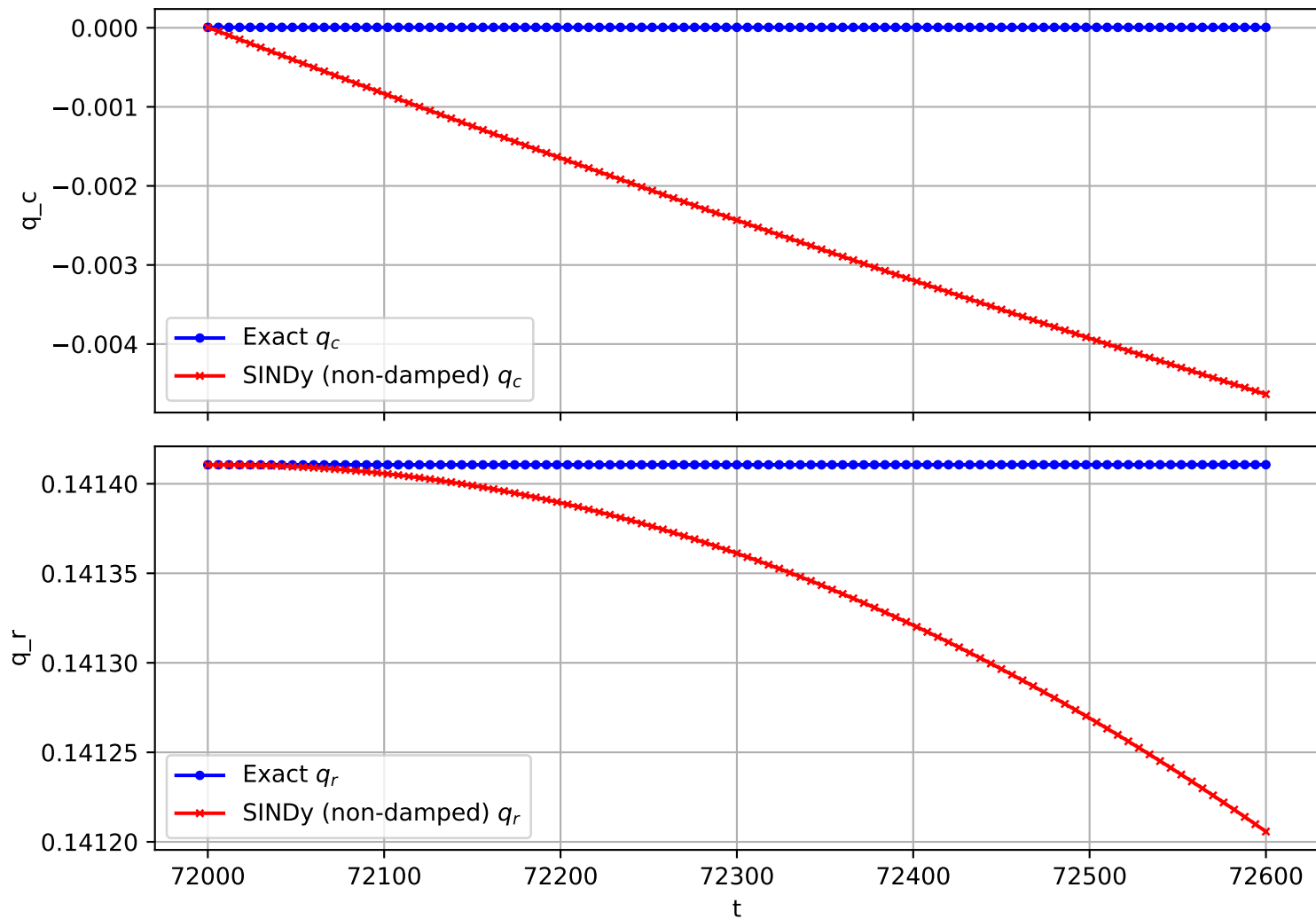
Trajectory 958 (non-damped)
