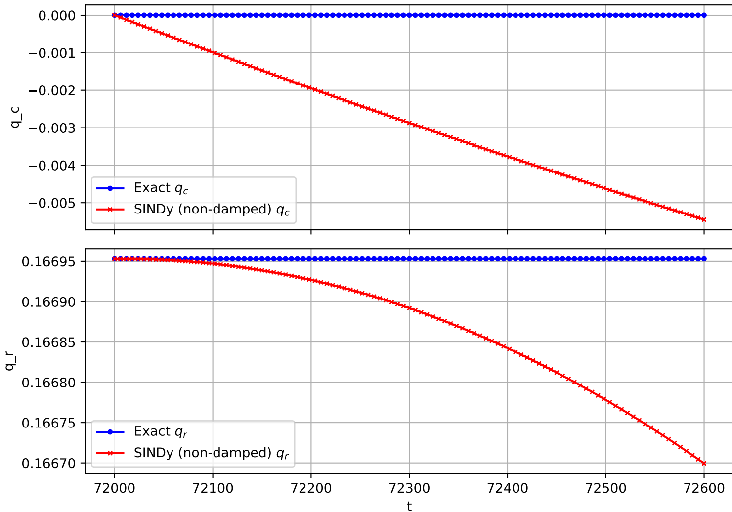
Trajectory 965 (non-damped)
