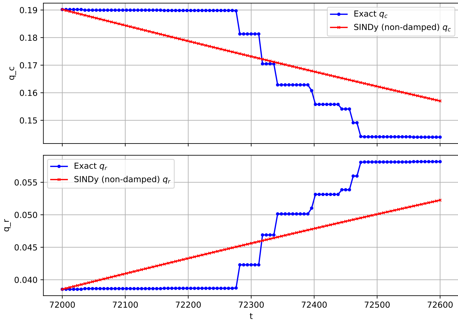
Trajectory 975 (non-damped)
