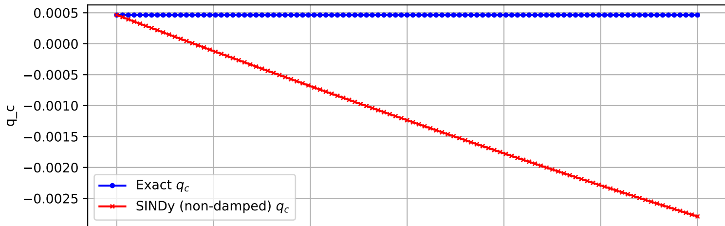
Trajectory 977 (non-damped)
