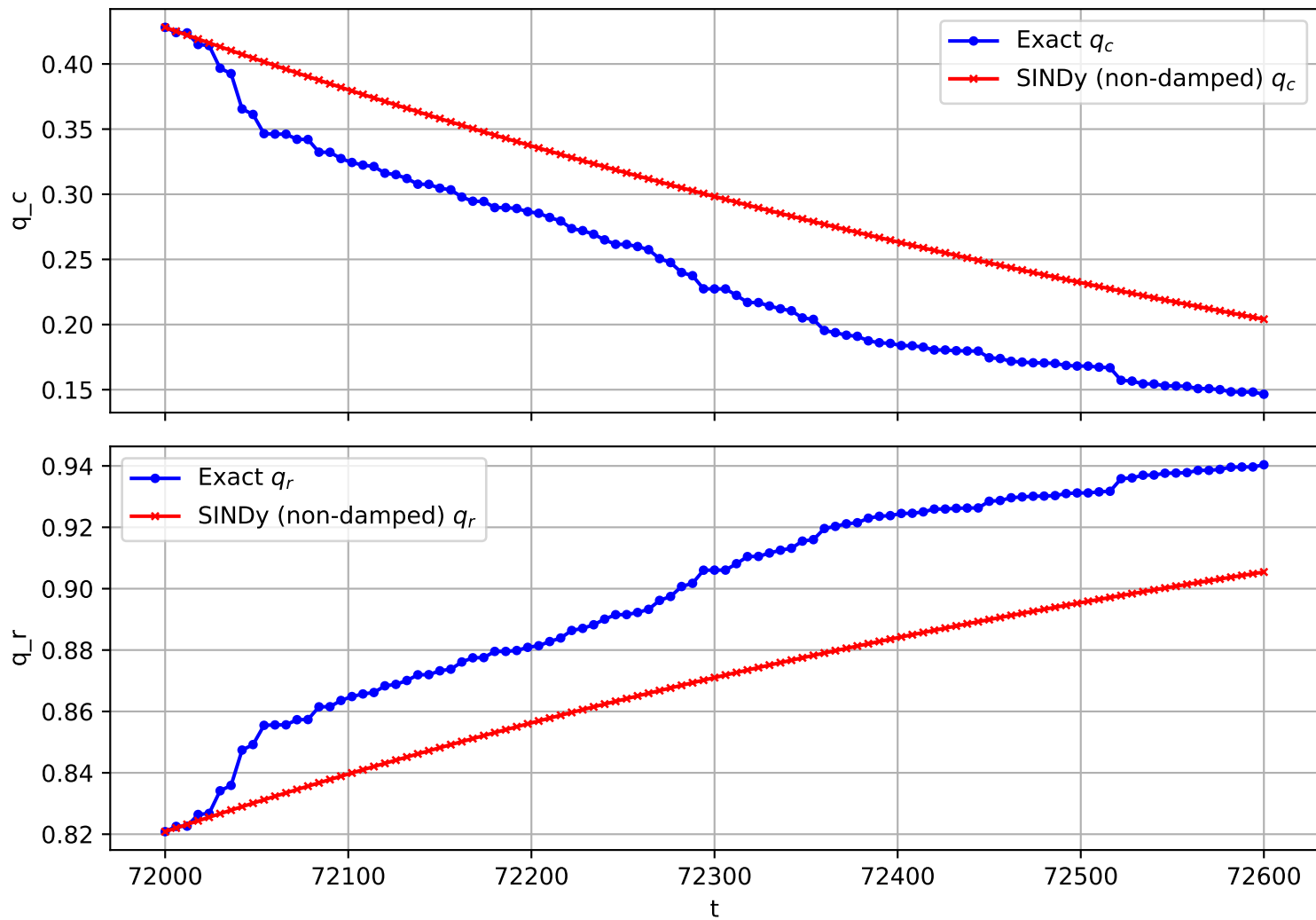
Trajectory 982 (non-damped)
