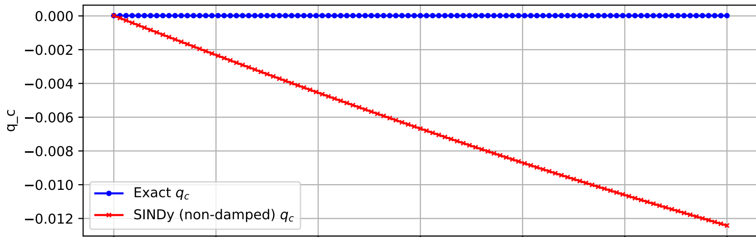
Trajectory 991 (non-damped)
