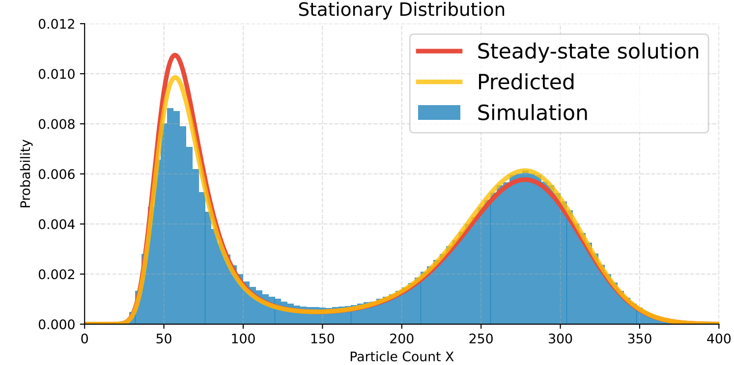
(f) Case 6: \gamma = 0.5477, D = 3000, \tau = 2.5 \times 10^{-7}
