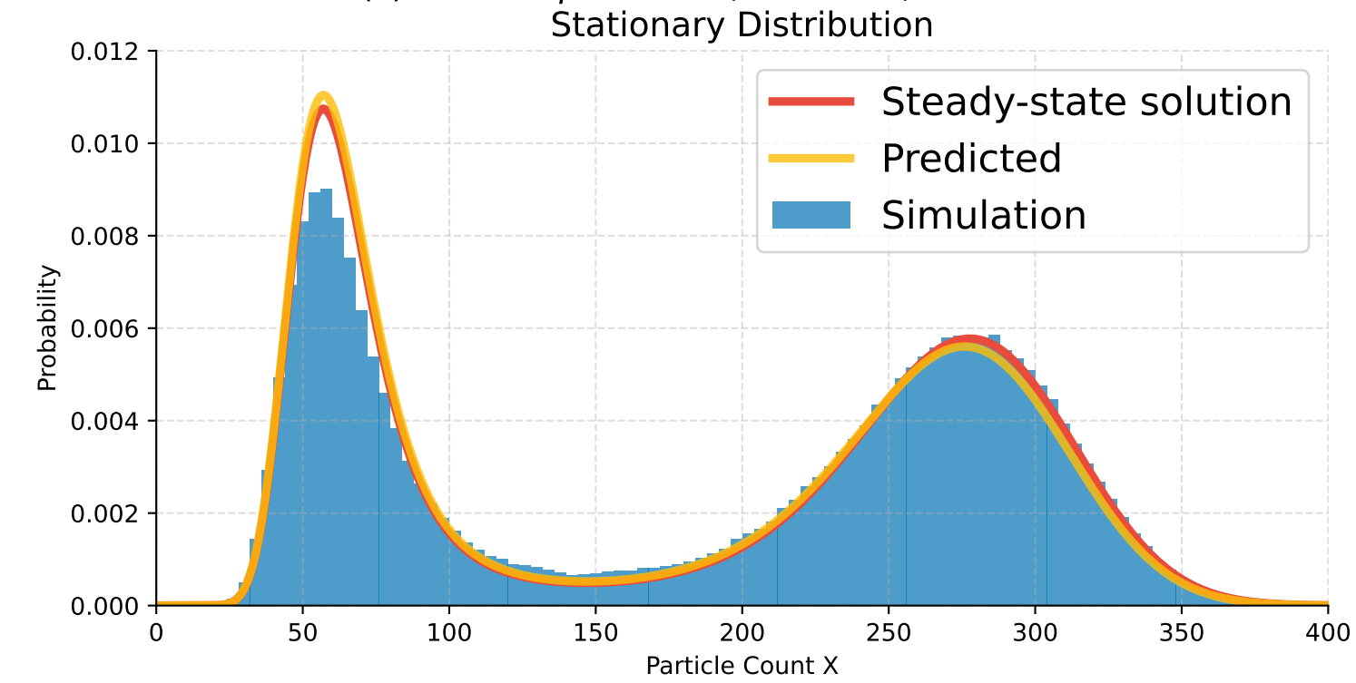
(c) Case 3: \gamma = 0.7746, D = 3000, \tau = 5 \times 10^{-7}
