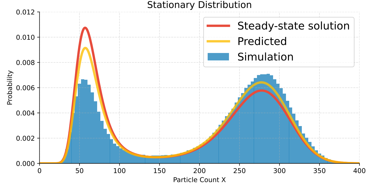
(e) Case 5: \gamma = 0.5477, D = 1500, \tau = 5 \times 10^{-7}
