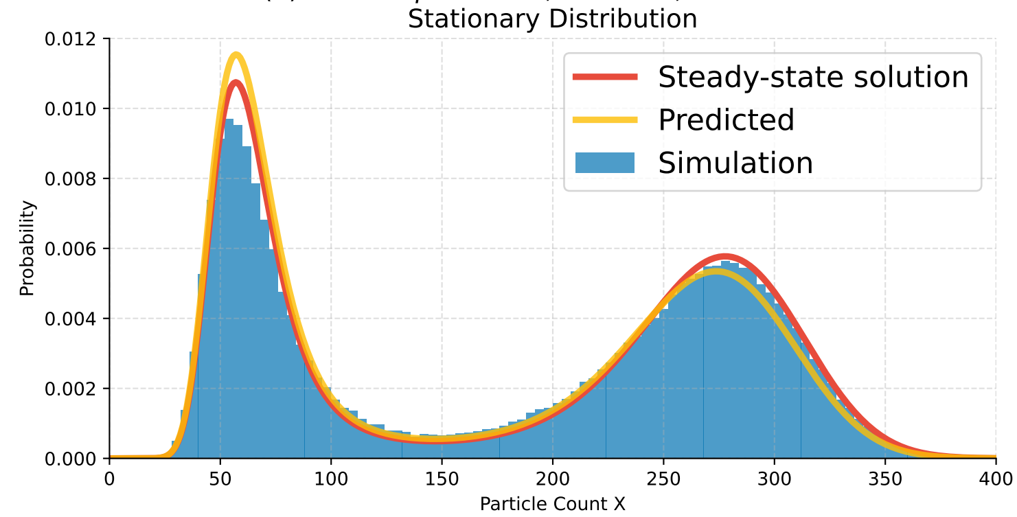
(b) Case 2: \gamma = 0.7746, D = 1500, \tau = 1 \times 10^{-6}
