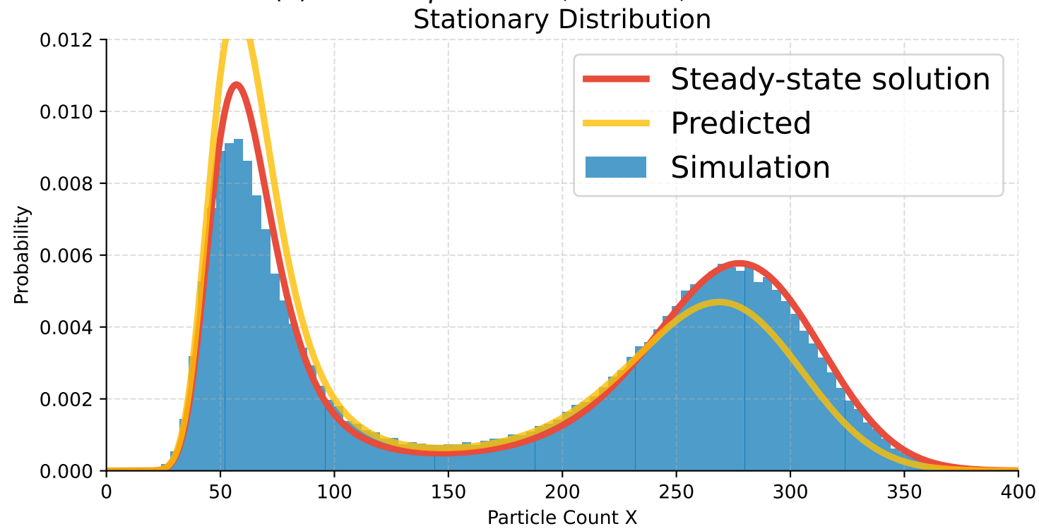
(a) Case 1: \gamma = 0.7746, D = 750, \tau = 2 \times 10^{-6}
