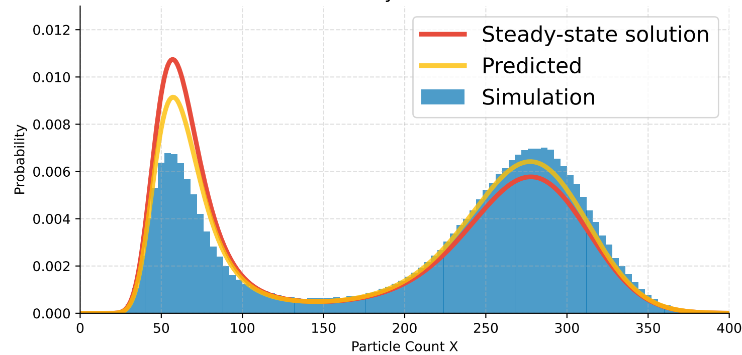
(e) Case 5: \gamma = 0.5477, D = 1500, \tau = 5 \times 10^{-7} Stationary Distribution
