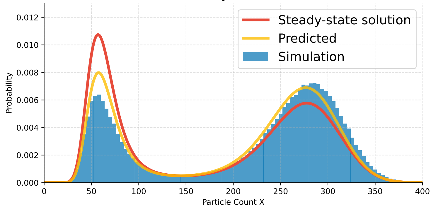
(d) Case 4: \gamma = 0.5477, D = 750, \tau = 1 \times 10^{-6} Stationary Distribution
