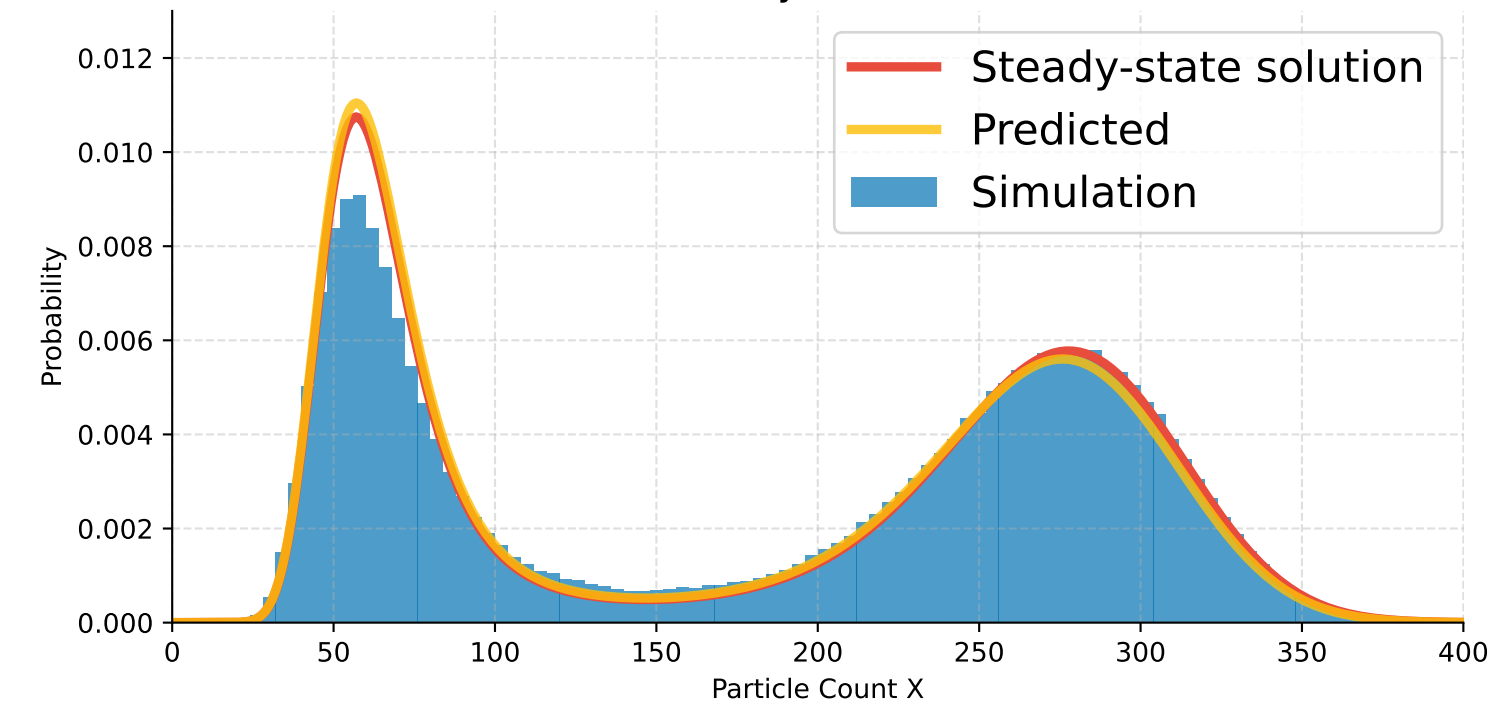
(c) Case 3: \gamma = 0.7746, D = 3000, \tau = 5 \times 10^{-7} Stationary Distribution
