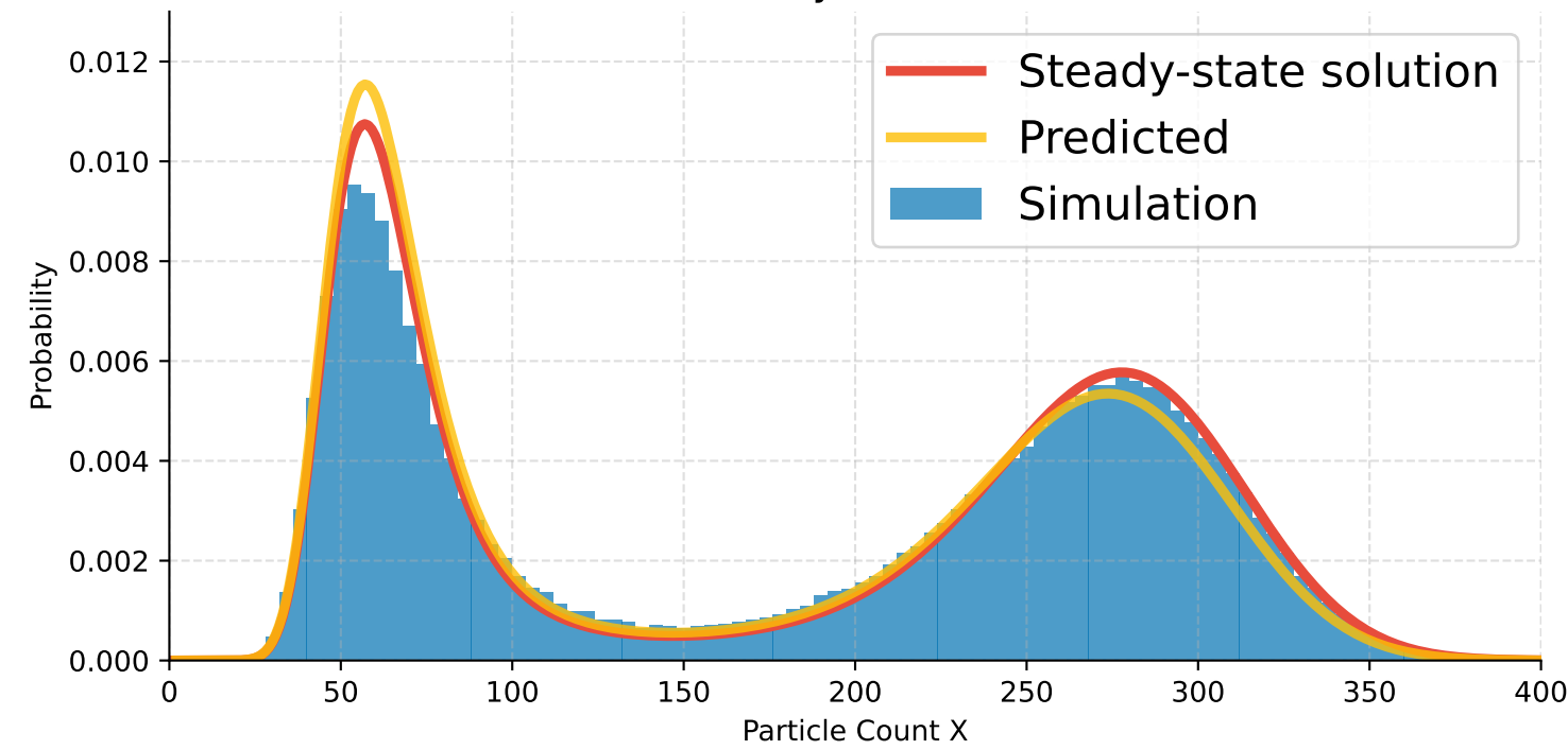
(b) Case 2: \gamma = 0.7746, D = 1500, \tau = 1 \times 10^{-6} Stationary Distribution
