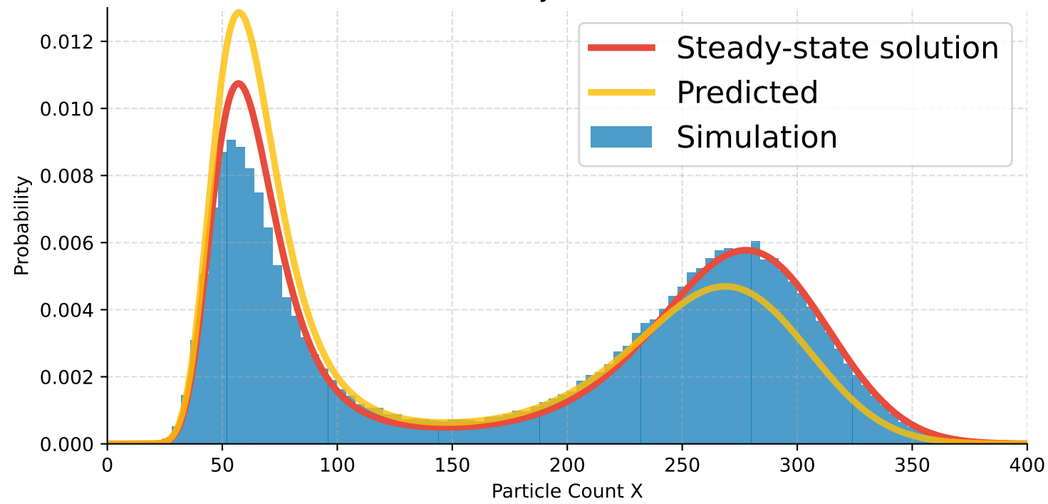
(a) Case 1: \gamma = 0.7746, D = 750, \tau = 2 \times 10^{-6} Stationary Distribution
