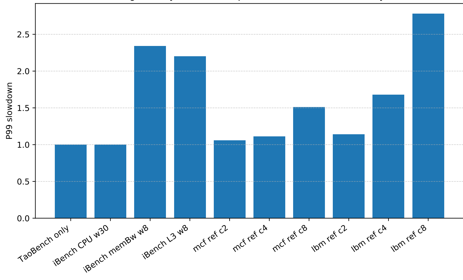
Stage 1: Key workload impact on TaoBench P99 latency
