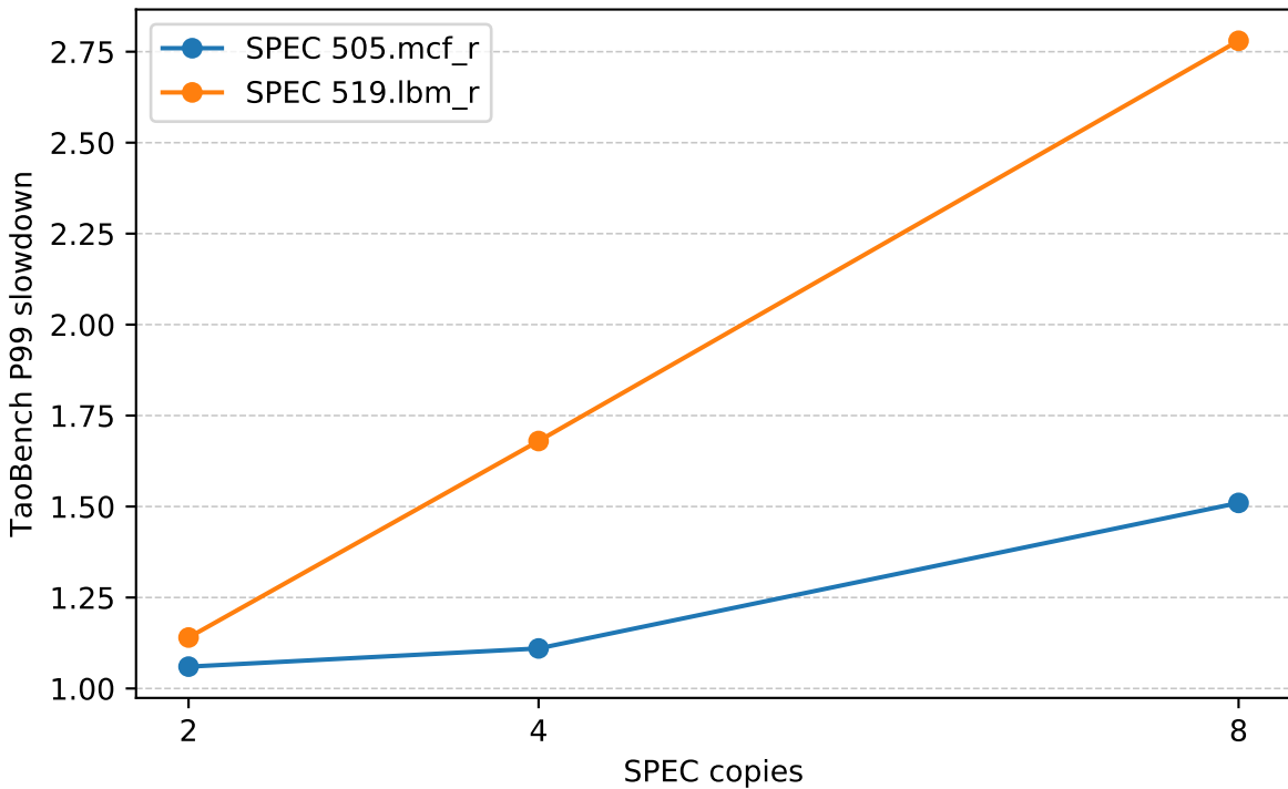
Stage 1: P99 slowdown vs. SPEC offline intensity
