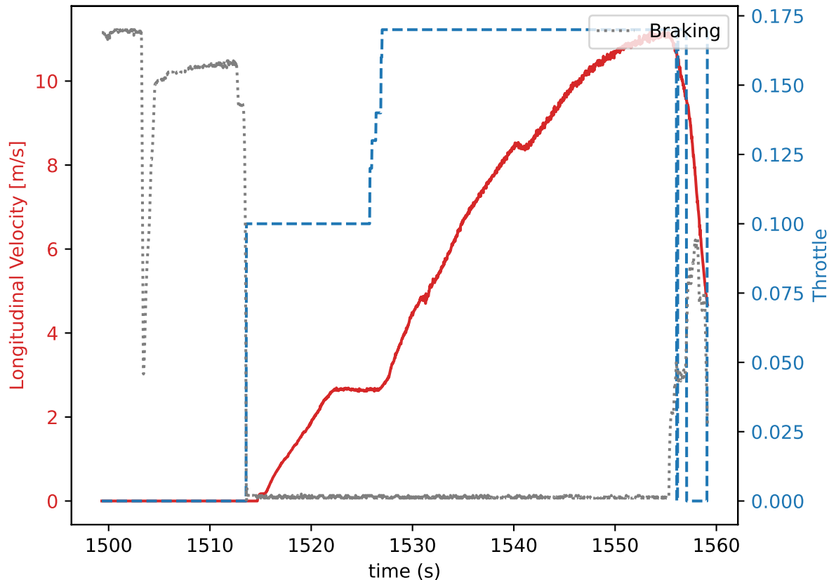
Linear throttle 10% to 17%
