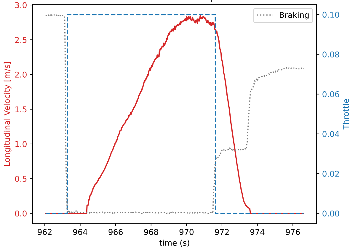
10% throttle step
