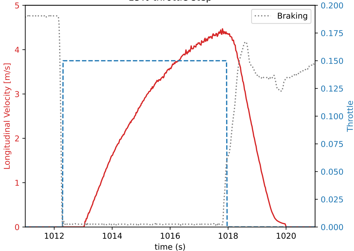
15% throttle step
