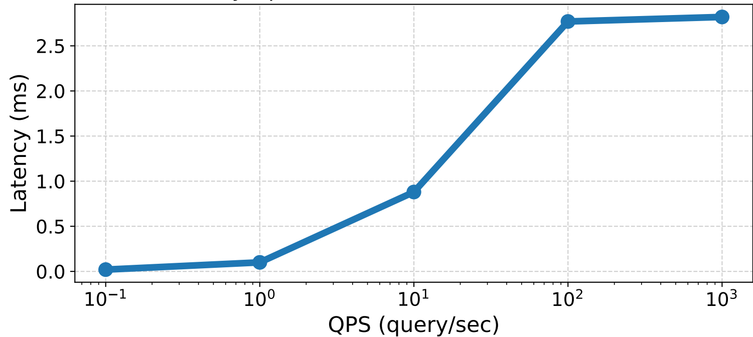
Policy Optimizer Runtime Overhead vs QPS
