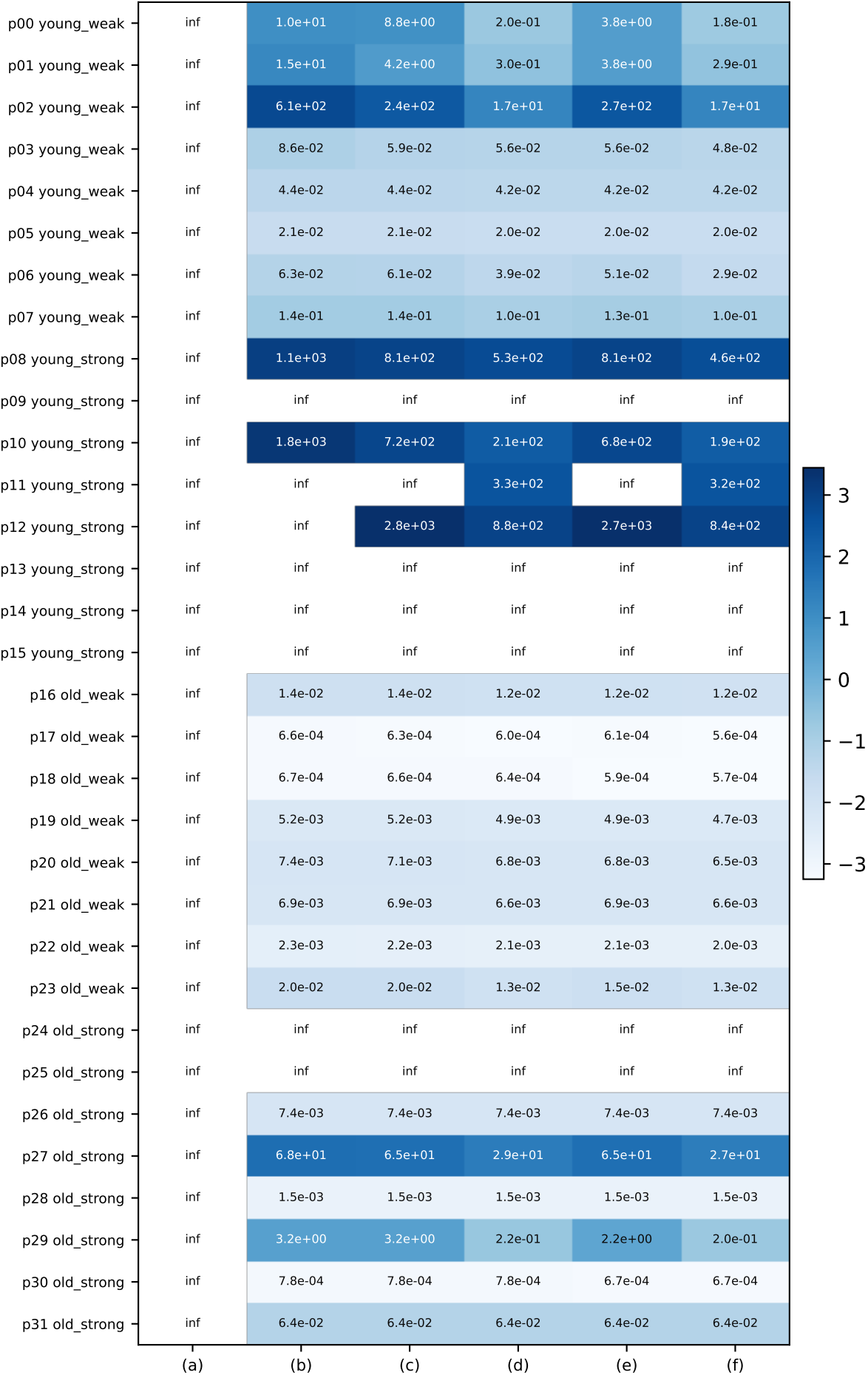
Cramer-Rao standard error of log T_r (with the seed columns) (log10 colour), T_r column scaled_c
