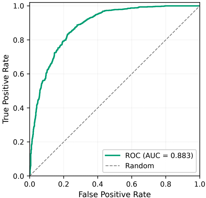
data1 — CatBoost (DL+ML stack)
