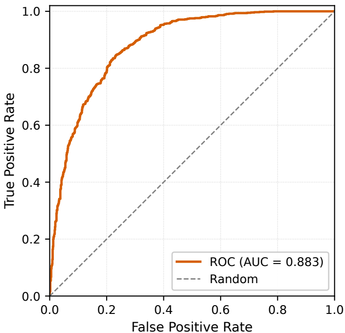
data1 — Ensemble (DL+ML stack)
