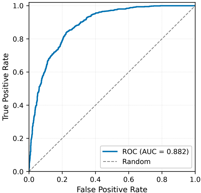
data1 — LightGBM (DL+ML stack)
