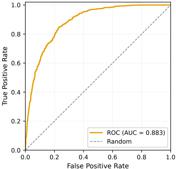
data1 — XGBoost (DL+ML stack)
