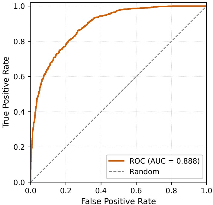
data2 — Ensemble (DL+ML stack)
