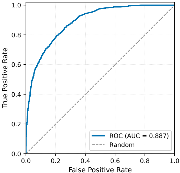
data2 — LightGBM (DL+ML stack)
