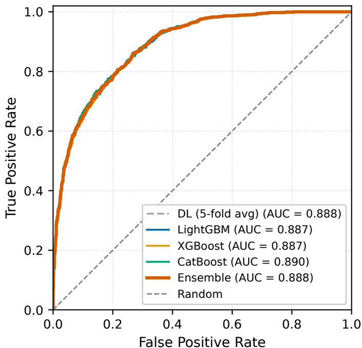
data2 — DL + ML stack
