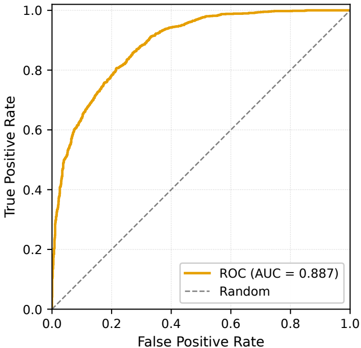
data2 — XGBoost (DL+ML stack)
