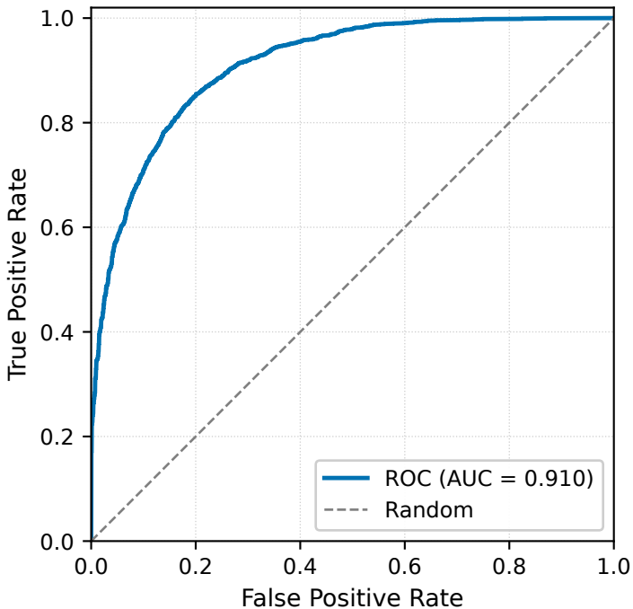
data3 — LightGBM (DL+ML stack)
