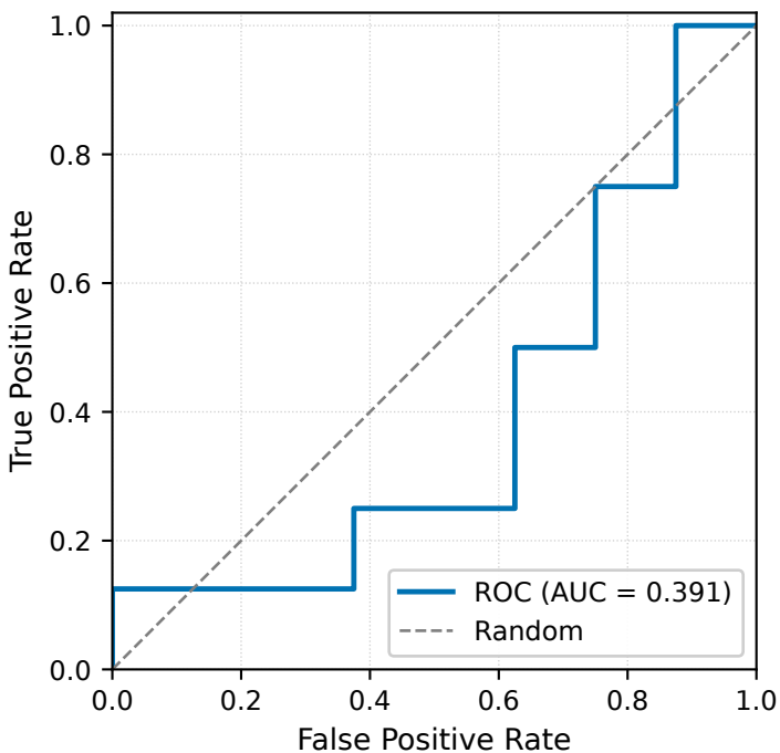
data1 — fold 5 (n=16)
