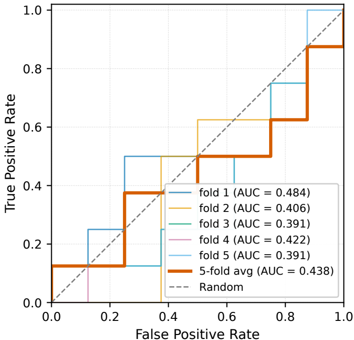
data1 — DL ROC on 16 samples
