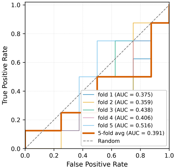
data2 — DL ROC on 16 samples
