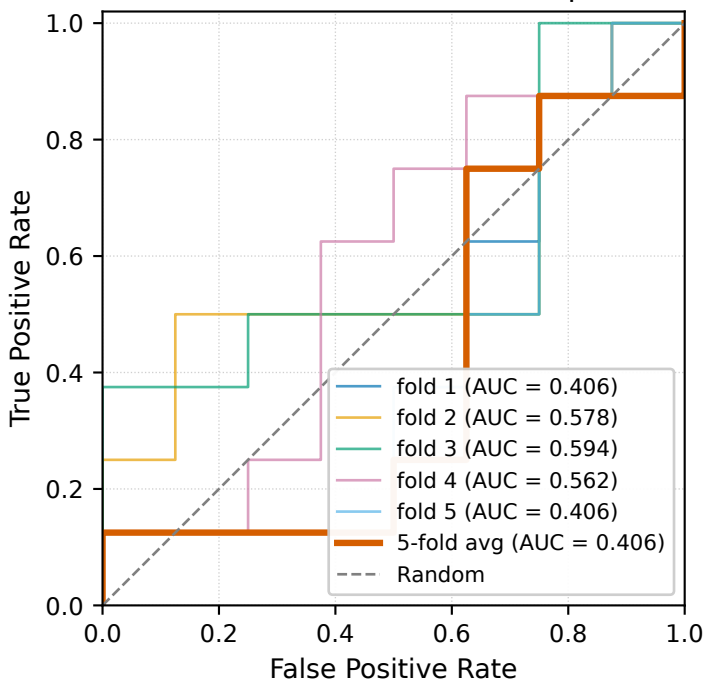
data3 — DL ROC on 16 samples
