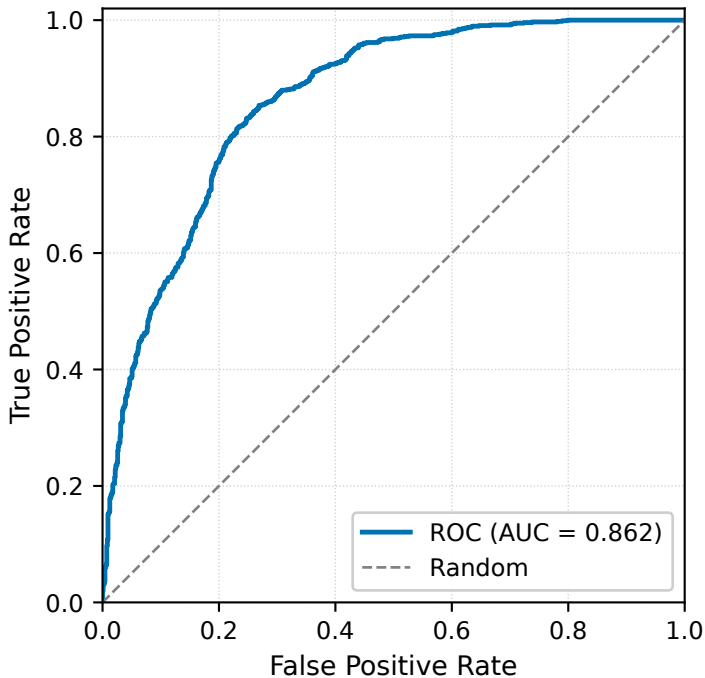
data1 — fold 1
