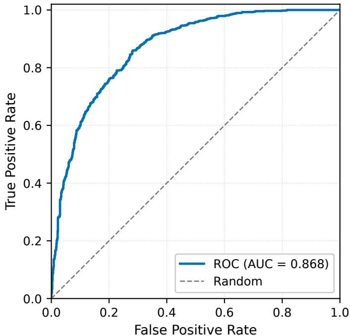
data1 — fold 4
