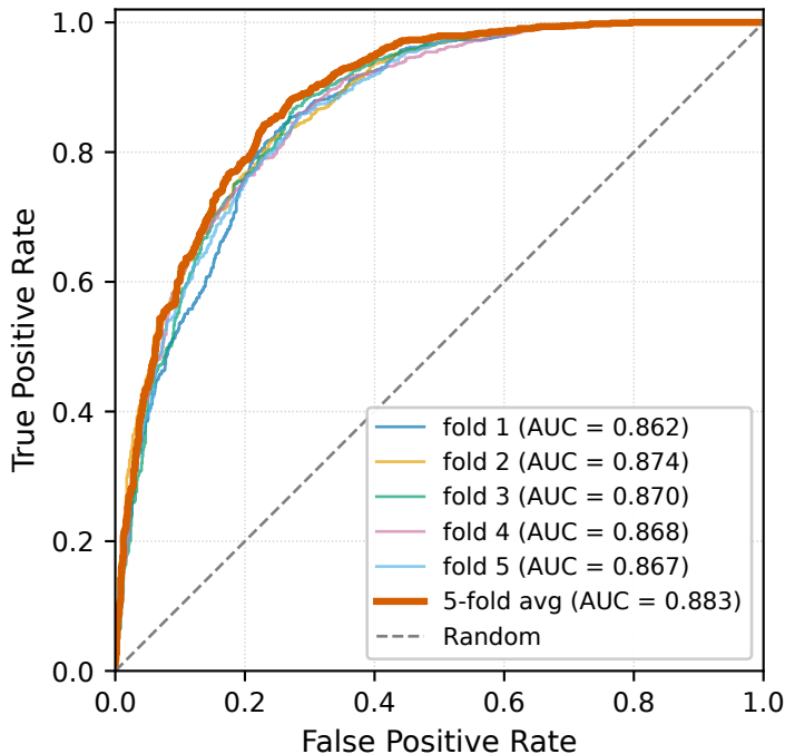
data1 — DL ROC (5 folds + avg)
