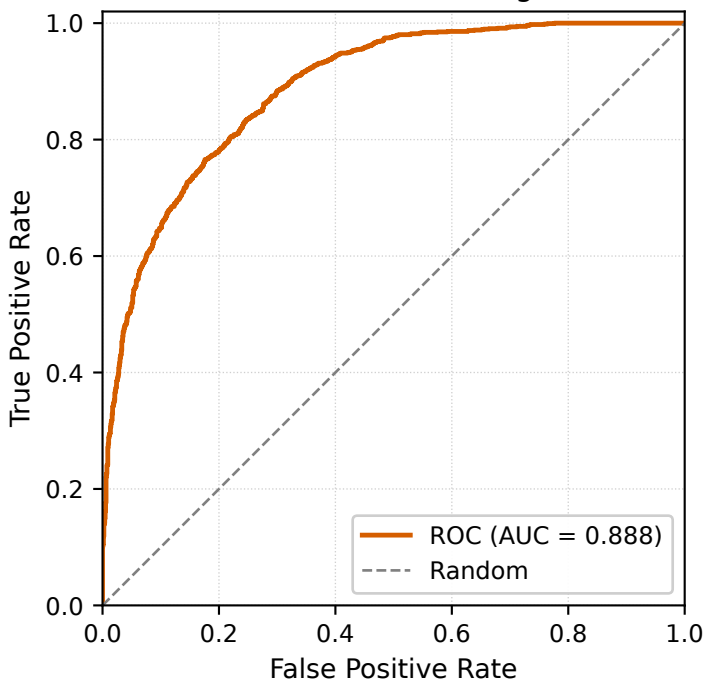
data2 — 5-fold avg
