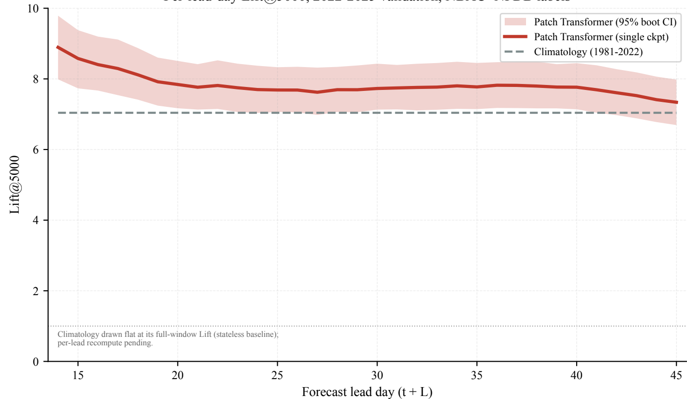
Per-lead-day Lift@5000, 2022-2025 validation, NBAC+NFDB labels
