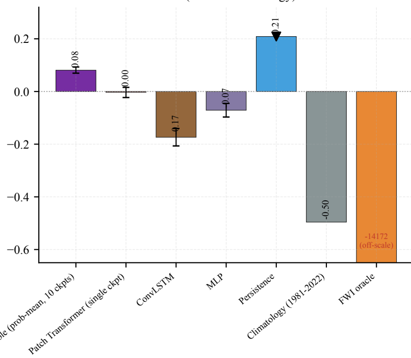
BSS (skill vs climatology)
