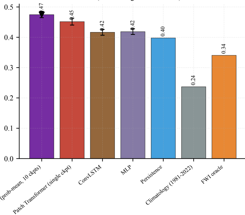
BSS (skill vs climatology)
