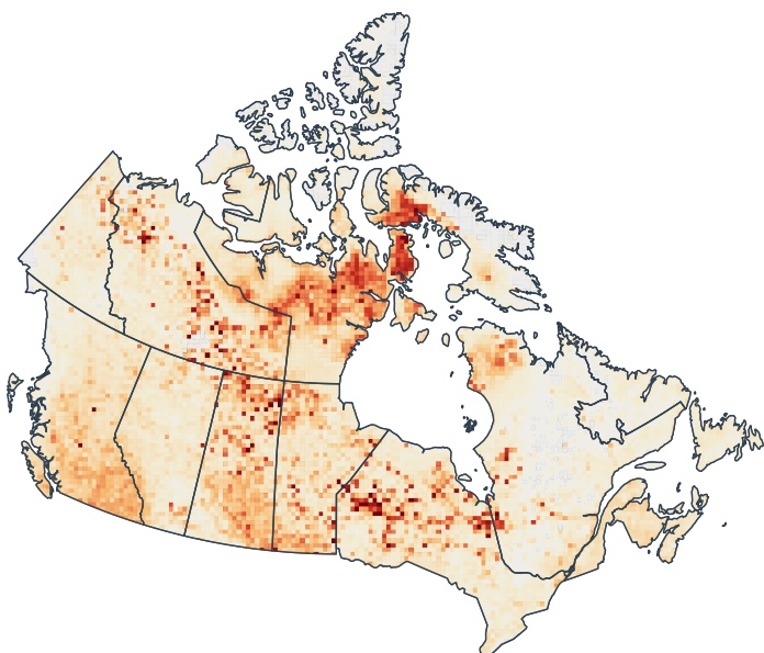
Forecast 2023-08-15, lead 30 d → 2023-09-14
