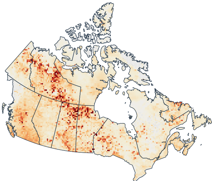
Forecast 2022-08-15, lead 30 d → 2022-09-14
