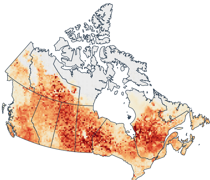
Forecast 2023-05-15, lead 30 d → 2023-06-14
