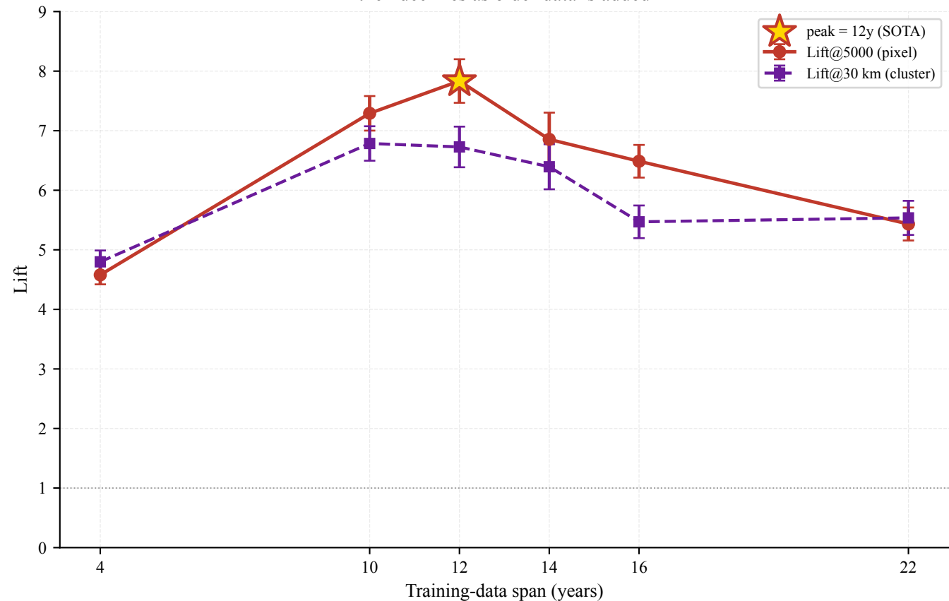
Data scaling: forecast skill peaks at 12 years, then declines as older data is added
