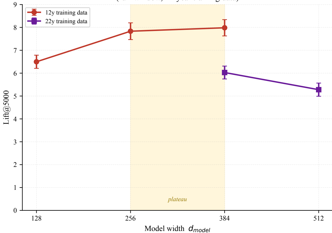
Model scaling: skill plateaus over d_{model} = 256 to 384 (full-window, 12-year training data)
