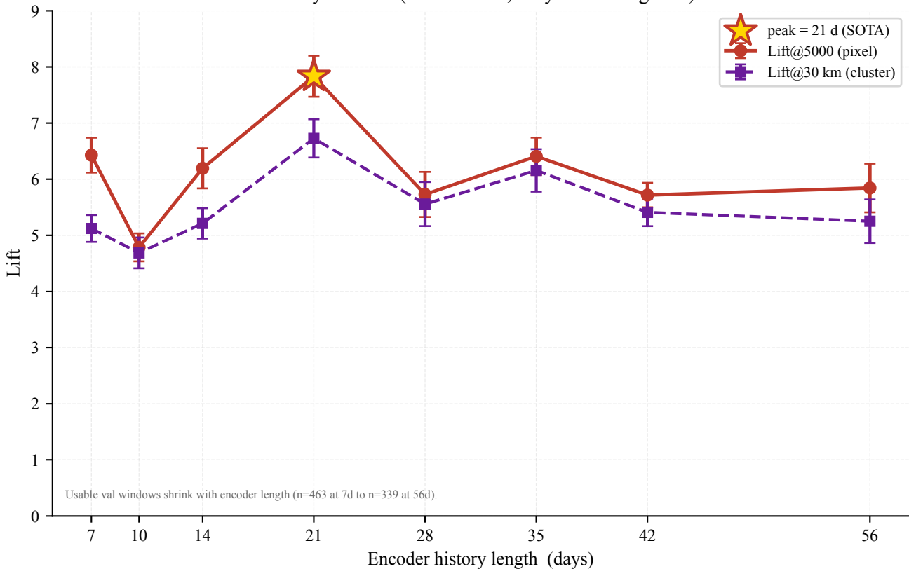
Encoder length: forecast skill peaks at a 21-day history window (full-window, 12-year training data)
