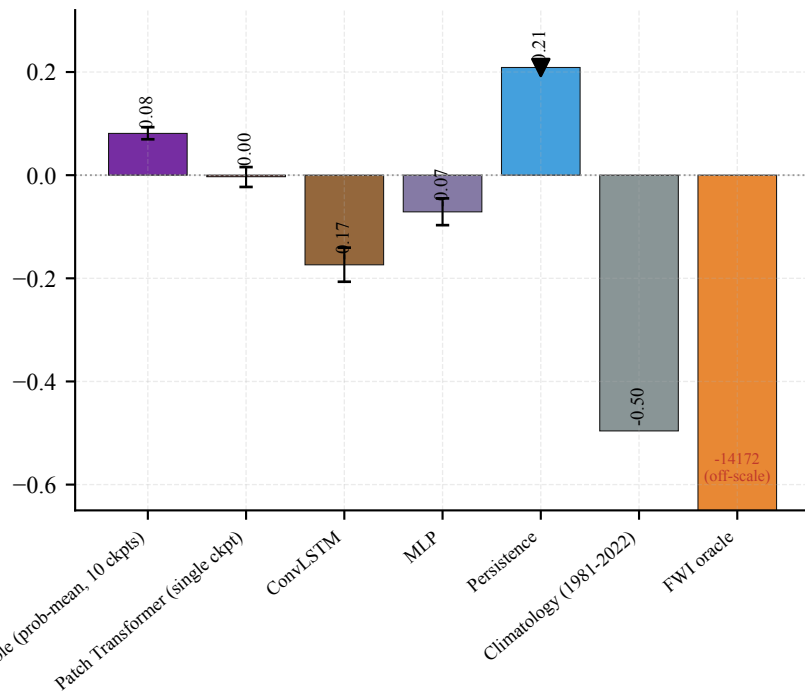
BSS (skill vs climatology)
