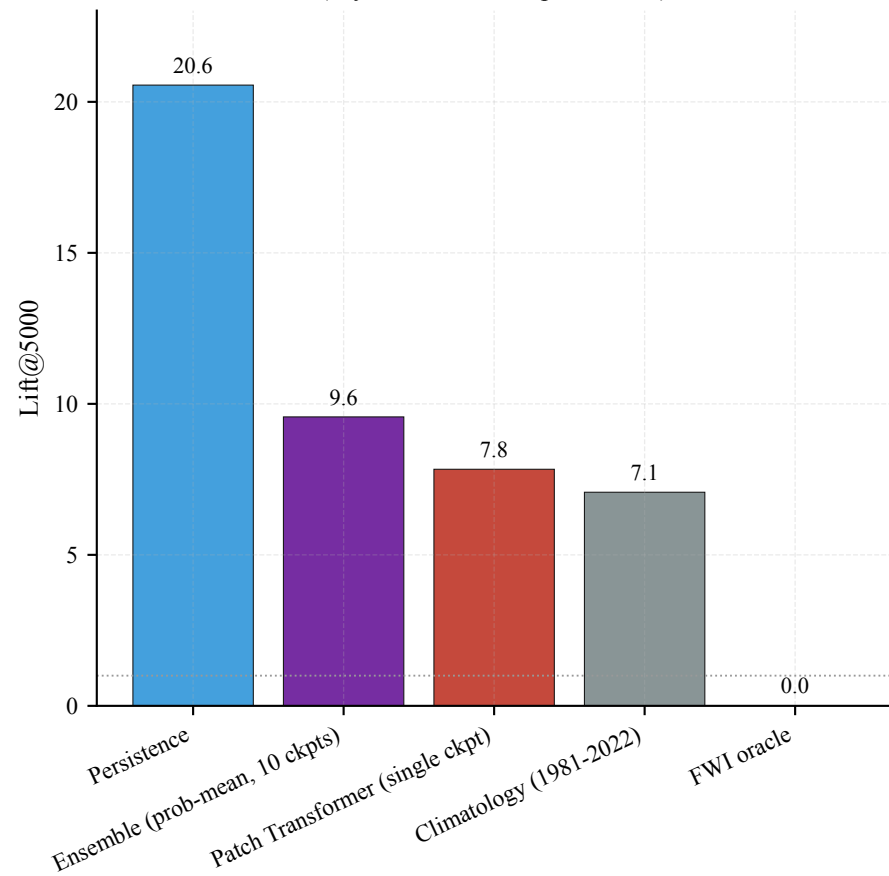
Standard Lift@5000 (any fire — rewards persistence)
