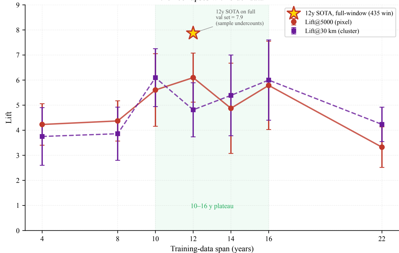
Data scaling: forecast skill peaks at 12 years, then collapses with older data
