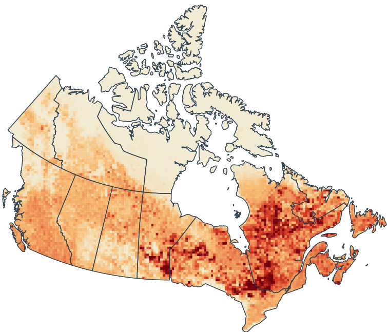
Lead 14 d → 2023-05-29
