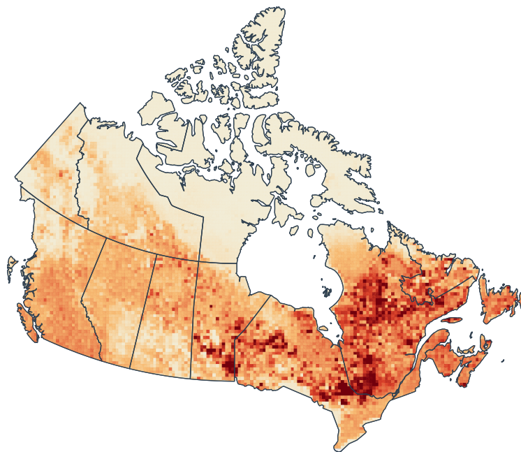
Lead 30 d → 2023-06-14
