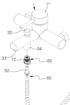
Implemented connection handle that can be easily connected to a faucet without tools
