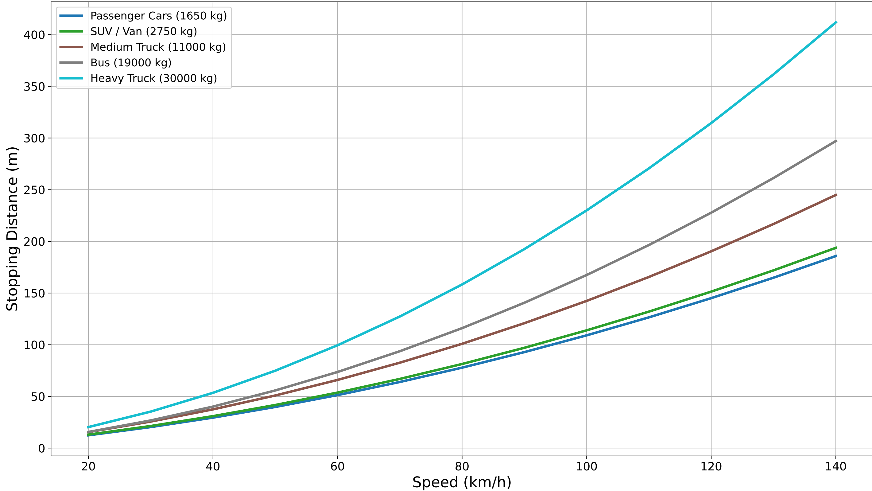
Stopping Distance by Vehicle Category (Day, Dry Conditions)
