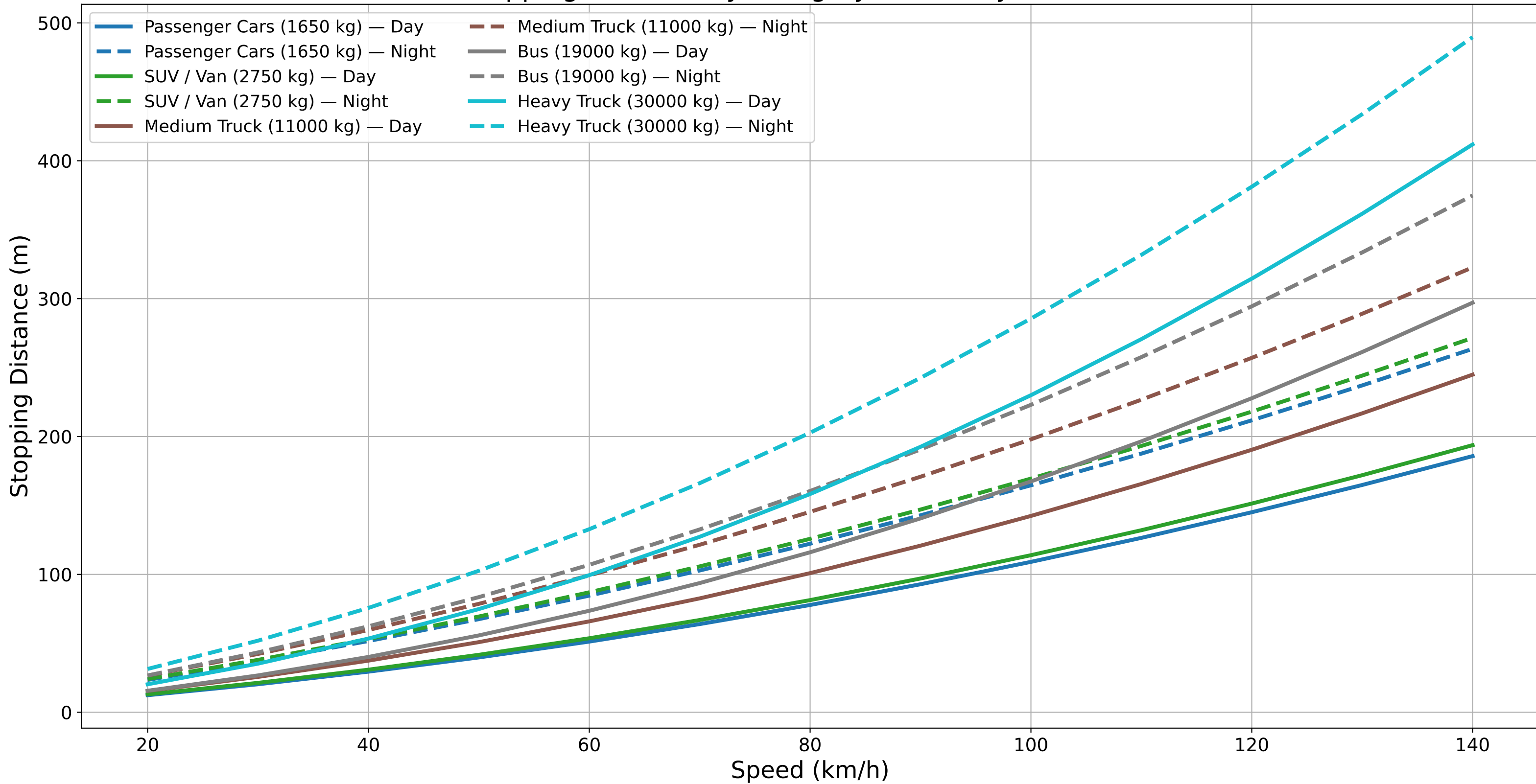
Stopping Distance by Category Under Dry Conditions
