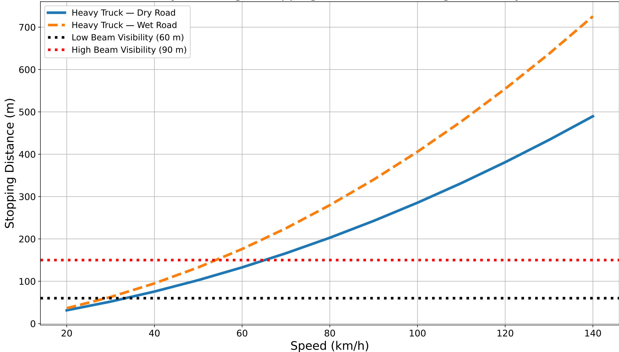
Heavy Truck Night Stopping Distance vs Headlight Visibility
