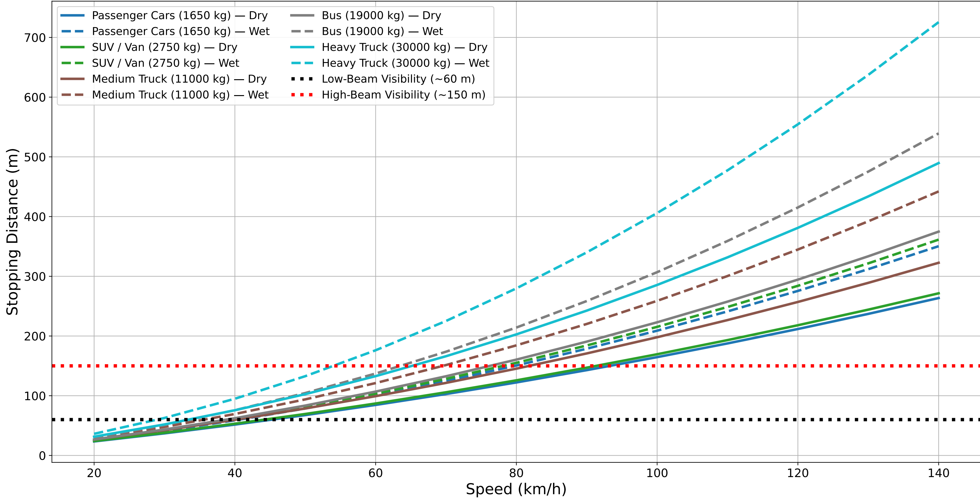
Nighttime Stopping Distance Relative to Headlight Visibility Thresholds
